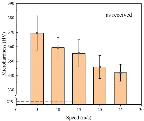
Figure 7 Surface microhardness variation at different grinding speeds
