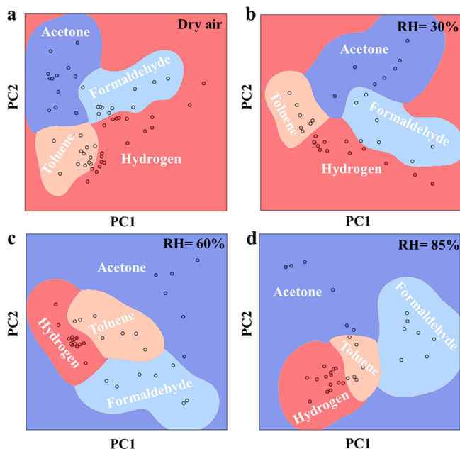
Figure 4. Gas classification of H_2 , formaldehyde, toluene, and acetone in different relative humidities: (a) dry air, (b) RH = 30%, (c) RH = 60%, (d) RH = 85%, employing support vector machine (SVM) algorithms.
