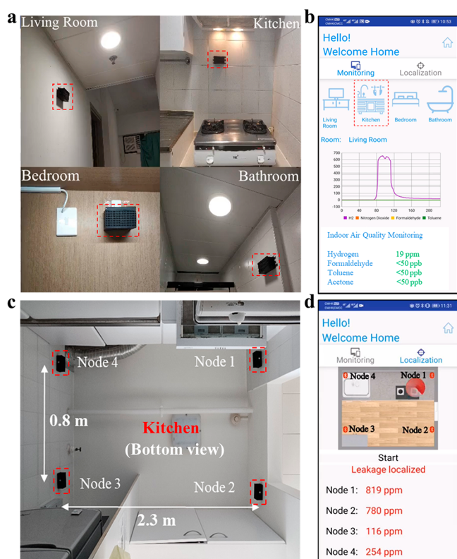
Figure 5. Smart home demonstration. (a) SINGOR systems deployed in the living room, kitchen, bedroom, and bathroom, respectively. (b) Cross-room real-time gas monitoring with the mobile app. (c) Four SINGOR systems deployed at the corners of the kitchen (bottom view). (d) Gas leakage source localization with red circle flashing shown in the mobile app.
