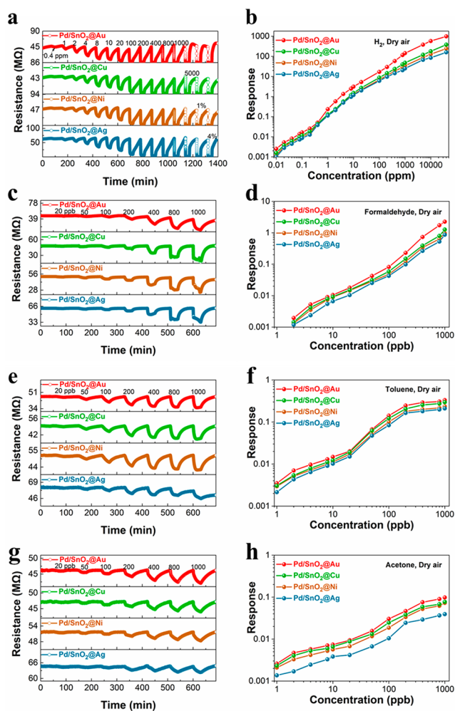
Figure 3. Room-temperature gas sensing properties (dry air) based on the 3D nanostructure gas sensor arrays. Sensing curves and response toward (a, b) H_2 from 10 ppb to 4%; (c, d) formaldehyde from 2 to 1000 ppb; (e, f) toluene from 1 to 1000 ppb; and (g, h) acetone from 1 to 1000 ppb.
