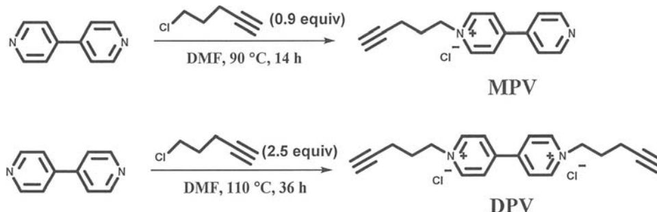
Fig. 1 Synthetic route of MPV and DPV. One-step synthesis of mono- or di-substituted viologen compounds.
