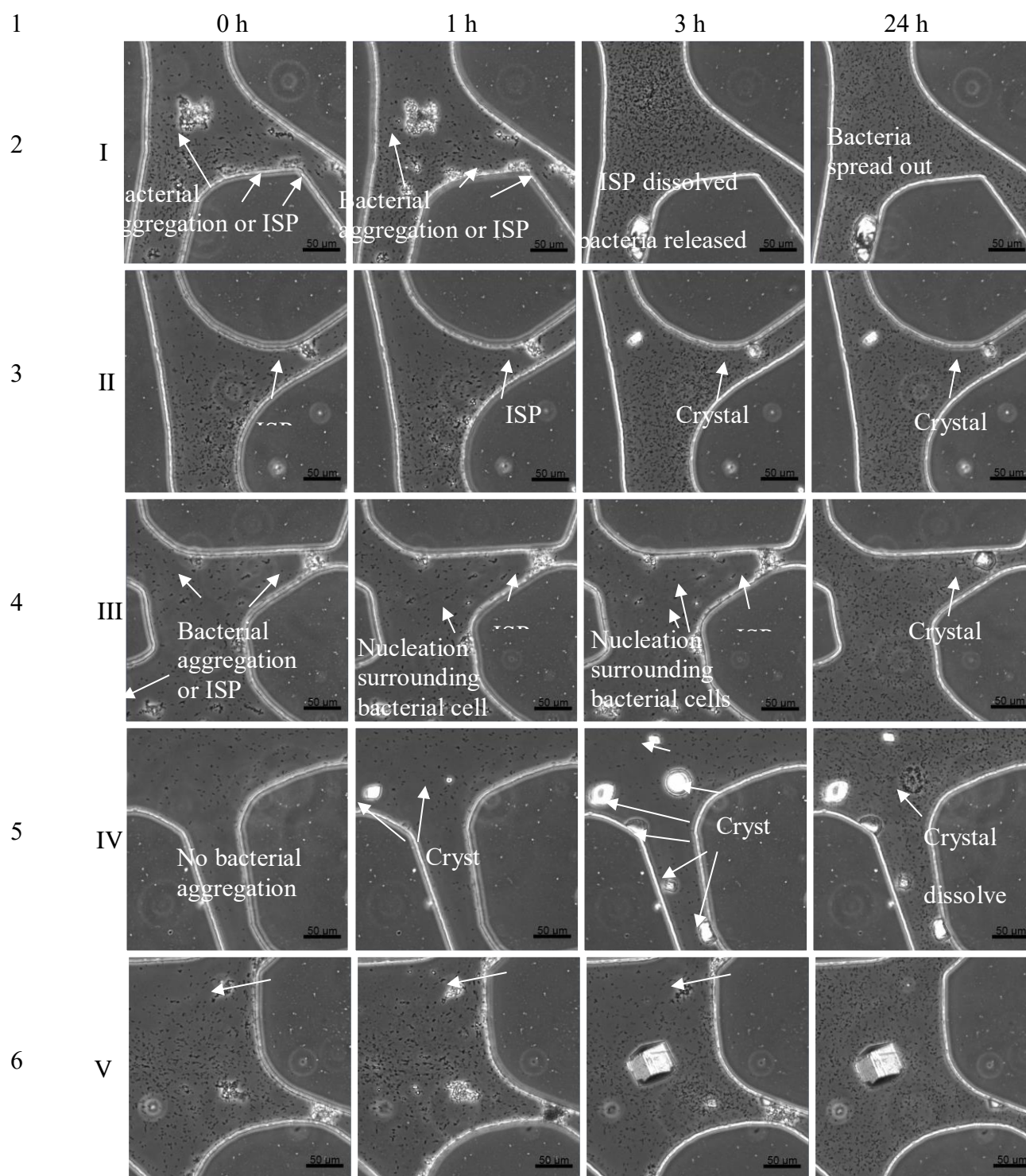
Fig. 12. Microscope images of five pores in the microfluidic chip (protocol 2) at 0, 1, 3 and 24 hours after the first injection of cementation solution
