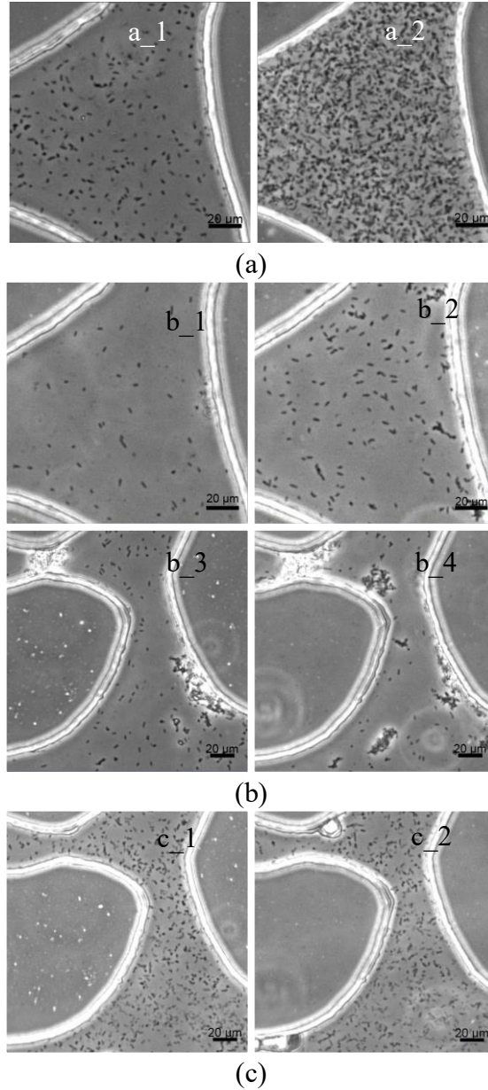
Fig. 11. (a) Microscope images of bacteria inside the central pore of the microfluidic chip after the injection of bacterial suspension (a_1) and after bacteria settling (a_2); (b) Microscope images of bacteria inside two central pores of the microfluidic chip after the injection of cementation solution injection at 0.5 ml per hour (b_1, b_3) and 0.05 ml per hour (b_2, b_4); (c) Microscope images of bacteria inside the central pore at 24 hours after cementation solution injection at 0.5 ml per hour (c_1) and 0.05 ml per hour (c_2).
