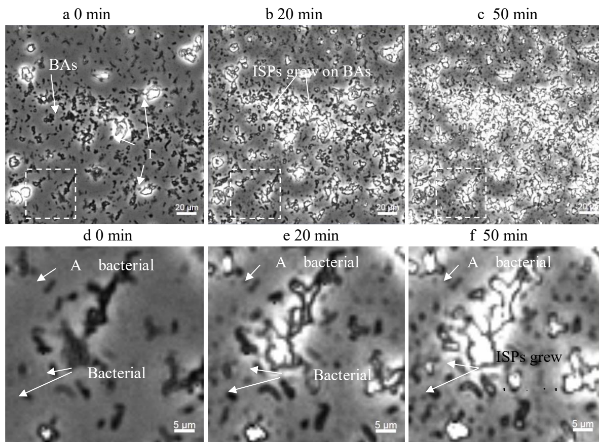
Figure 6 Microscope images showing the precipitation of irregular-shaped \text{CaCO}_3 crystals and the fixation of bacterial cells during the precipitation process. (a) at 0 min, bacterial aggregates (BAs) and irregular-shaped precipitates (ISP) formed; (b and c) ISPs formed on bacterial aggregates; (d and e) three bacterial cells shown by arrows; (f) at 50 mins, ISPs grew on the bacterial cells shown by the bottom two arrows but did not form on the bacterial cell shown by the top arrow
