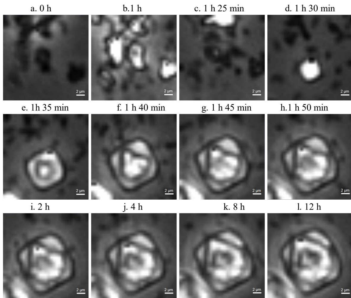
Figure 10 Microscope images showing growth of a rhombohedral \text{CaCO}_3 crystal. (a-c) events preceding the formation of the crystal; (d-l) crystal formation and growth.
