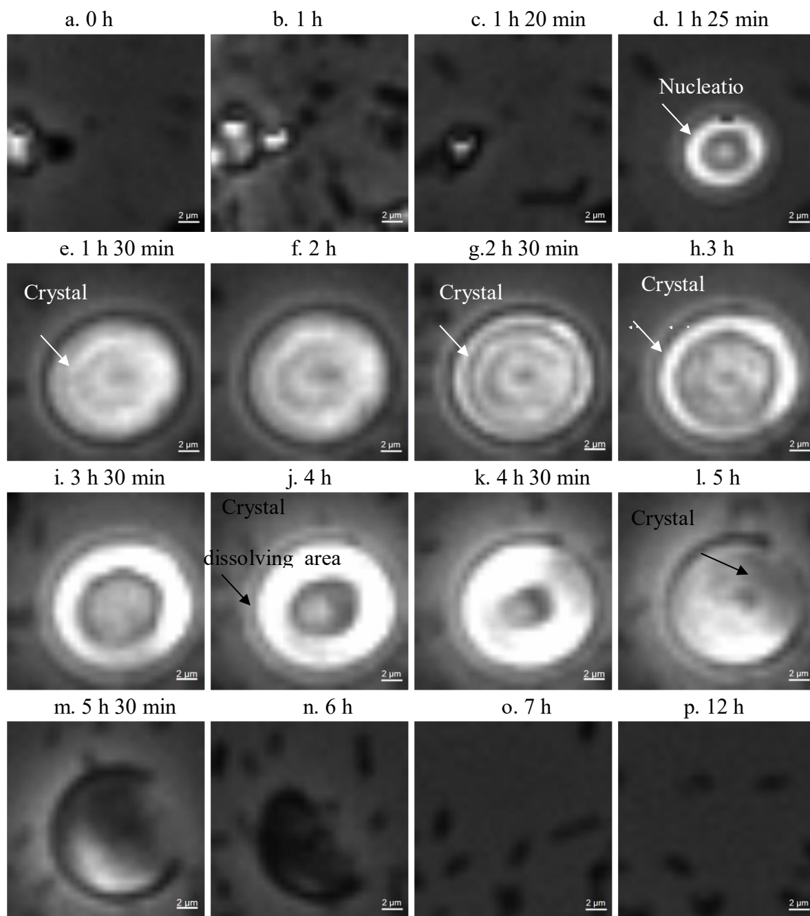
Figure 9 Microscope images showing the growth and dissolution of a spherical \text{CaCO}_3 crystal. (a-c) events preceding the formation of the crystal; (d-g) crystal growth phase; (h-p), dissolution of the crystal, scale bar 2 \mu\text{m} .
