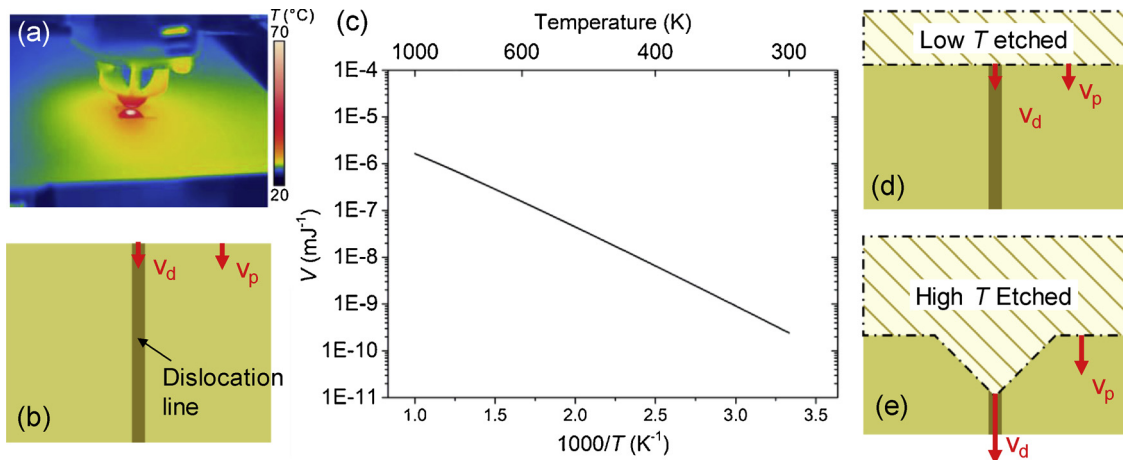
Fig. 3. a) Thermal image of the substrate during CCP etching. b, d, e) Schematic of 4H-SiC with a threading dislocation line (b) before etching, (d) after low temperature etching and (e) high temperature etching. c) The Arrhenius style plot of V-Temperature.
