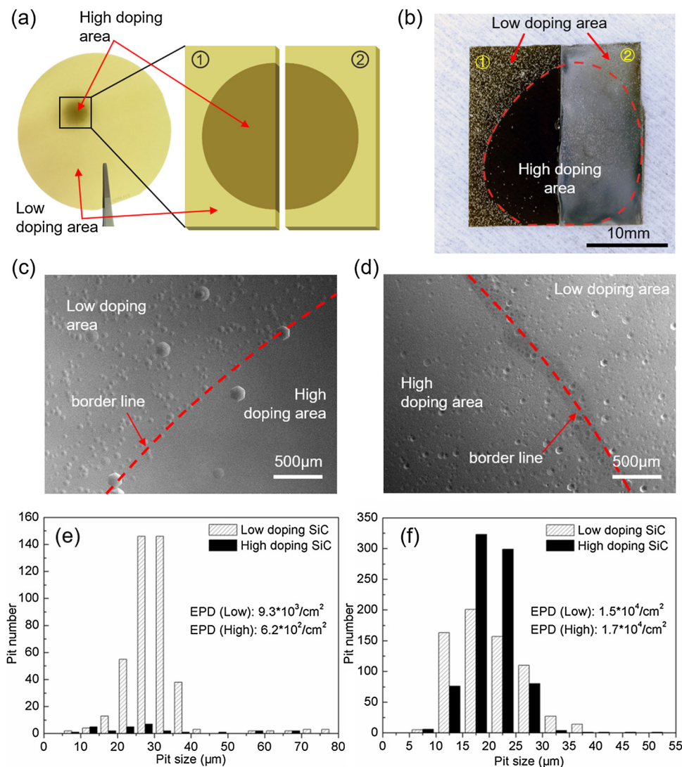
Fig. 6. a) Optical photo of the SiC wafer used (left) and the schematic of the two samples cut off from that wafer (right). b) Optical photo of the samples after conventional molten KOH etching and ICP etching respectively. c, d) SEM images for the boundary area between low doping area and high doping area of SiC etched by (c) conventional method and (d) plasma etching method. e, f) Size distribution of etching pits of the low and high doping areas for SiC samples processed by (e) molten KOH etching and (f) plasma etching.
