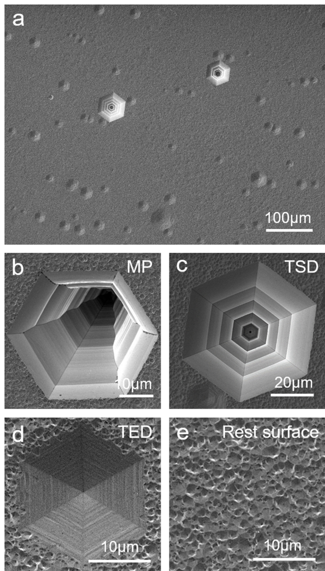
Fig. 5. a) SEM image of the ICP etched surface of SiC and the close-up SEM image of b) MP; c) TSD; d) TED and e) the rest surface.
