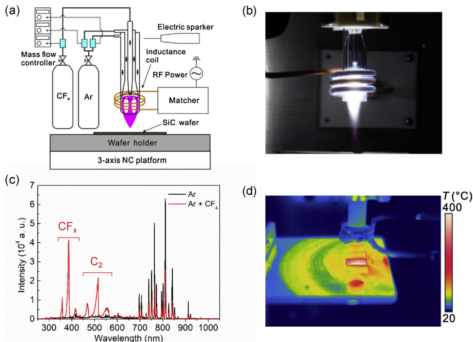
Fig. 4. a) Schematic diagram of experimental setup for ICP plasma etching. b) optical photo of the ICP jet. c) OES spectra of the ICP jet without and with CF 4 addition. d) thermal image of the substrate during ICP etching.
