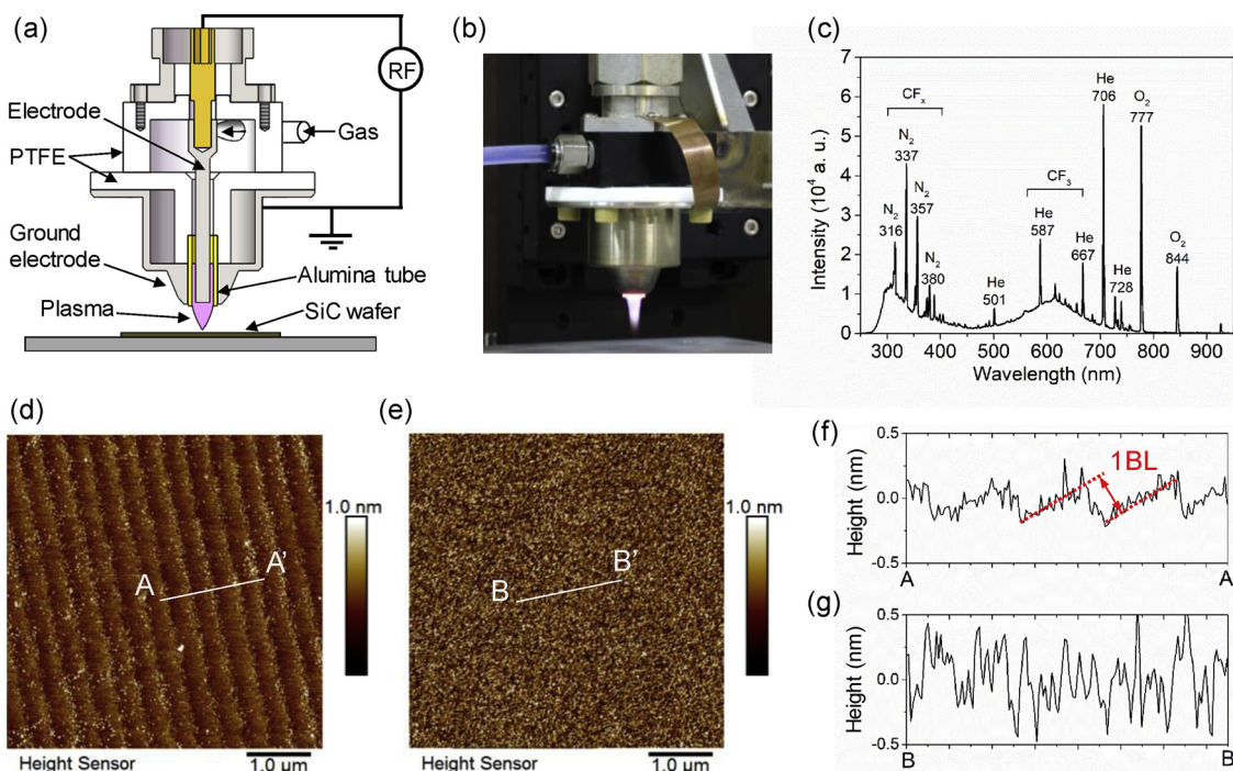
Fig. 2. a) Schematic diagram of experimental setup for CCP jet etching. b) optical photo of the CCP jet. c) OES spectra of the CCP jet. d, e) AFM images of the SiC of 4H-SiC sample (d) before and (e) after CCP etching. f, g) Cross sectional profiles along A-A' and B-B' respectively.
