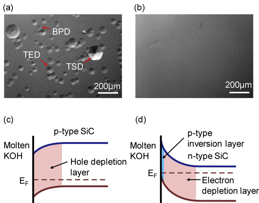
Fig. 1. a, b) SEM images of the molten KOH etched surface of low doping SiC and high doping SiC. c, d) Band structure schematics of 4H-SiC/molten KOH interface for p-type SiC and high doping n-type.
