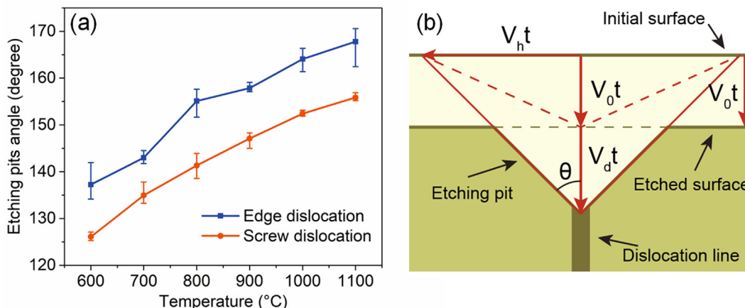
Fig. 7. (a) The relationship between the etch pit angle and the etching temperature for edge dislocation and screw dislocation after etching at 600–1100 °C for 2 min, and (b) the schematic of the etch pit formation.
