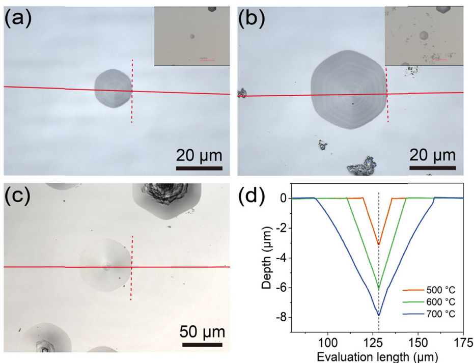
Fig. 6. In-situ CLSM image of an edge dislocation after etching for 1 min at: (a) 500 °C, (b) 600 °C, (c) 700 °C; (d) the cross-sectional profile of (a–c) along the solid red line. The angles are 137.8°, 139.0° and 153.9°, respectively.
