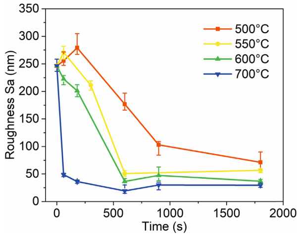
Fig. 4. Surface roughness of the Si-face of 4H-SiC after etching at 500–700 °C for 0–30 min.
