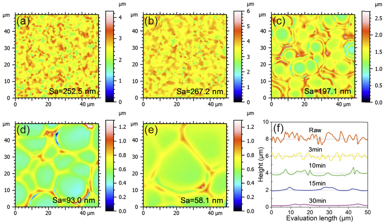
Fig. 3. White light interferometer image of the Si-face after etching at 500 °C for: (a) 0 min (the raw SS-SiC surface), (b) 3 min, (c) 10 min, (d) 15 min, (e) 30 min; (f) the cross-sectional profiles of the surface (a–e), respectively.
