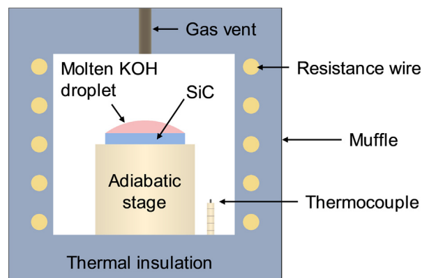
Fig. 1. Schematic diagram of the experimental setup for KOH etching.
