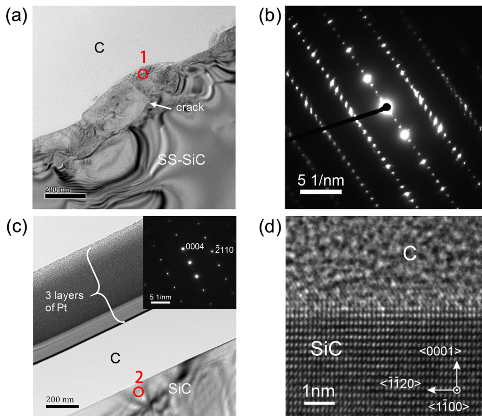
Fig. 10. (a) The TEM image of the SS-SiC sample, (b) the SAED pattern of spot 1 in (a), (c) TEM image of the sample after 2 min KOH etching under 800 °C, the insert is the SAED of spot 2; (d) the HRTEM of (c).
